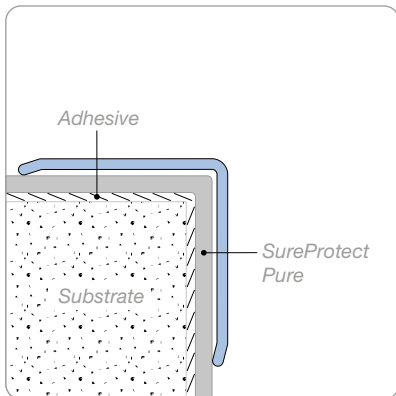
185 Series Stainless Steel Corner Guard Illustration is not to scale.
