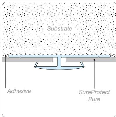
1 Part Joiner Trim - SPP/1PJ
