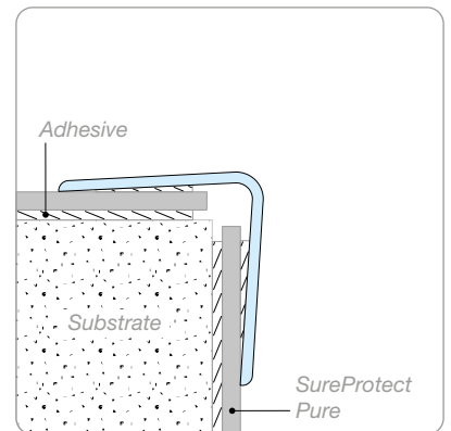
External Angle - SPP/EA50
