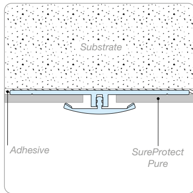
2 Part Joiner Trim - SPP/2PJ
