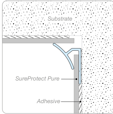
Internal Corner - SPP/ICS
