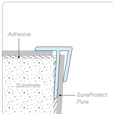
External Corner - SPP/EC
