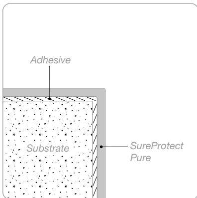
Thermoformed External / Internal Corner Formed on-site during installation.
