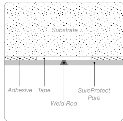
Weld Rod - WR
