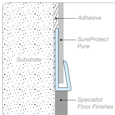
1 Part Copper Trim - SPP/1PC
