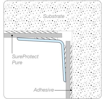
Internal Angle - SPP/IA50
