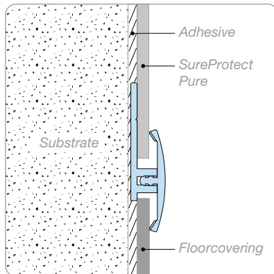
2 Part Transition Trim - SPP/2PT
