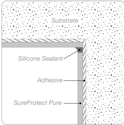
Silicone Sealant - SC310
