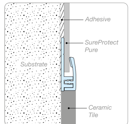
2 Part Copper Trim - SPP/2PC
