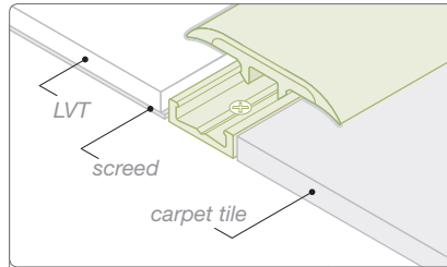
TT35/AFT15 LVT to carpet tile.
