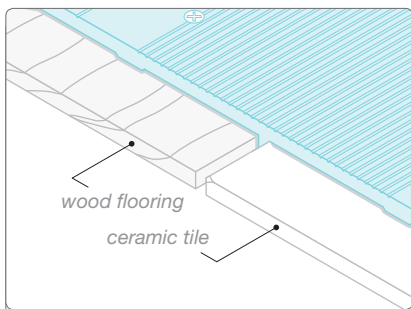
ACS470S wood flooring to ceramic tile.
