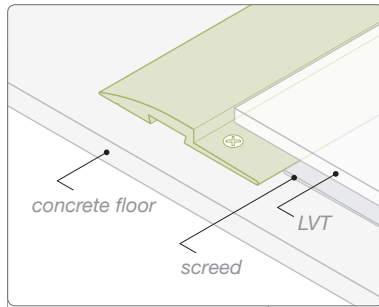
TA16 LVT to concrete floor.
