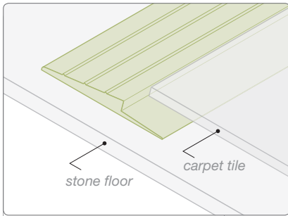
PCR632 carpet tile to stone floor.
