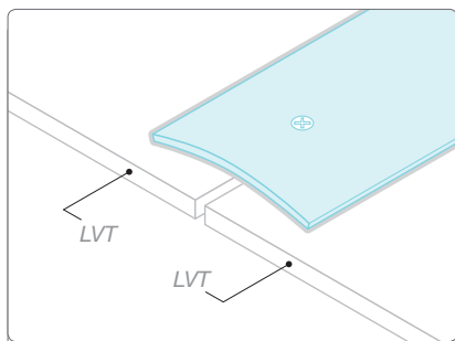
SCSM451 LVT to LVT.
