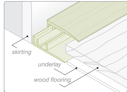
KB587LH wood flooring to skirting.
