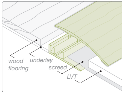
KA586LH wood flooring to LVT.
