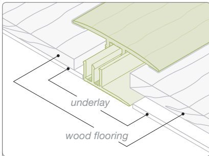
KC588H wood flooring to wood flooring.
